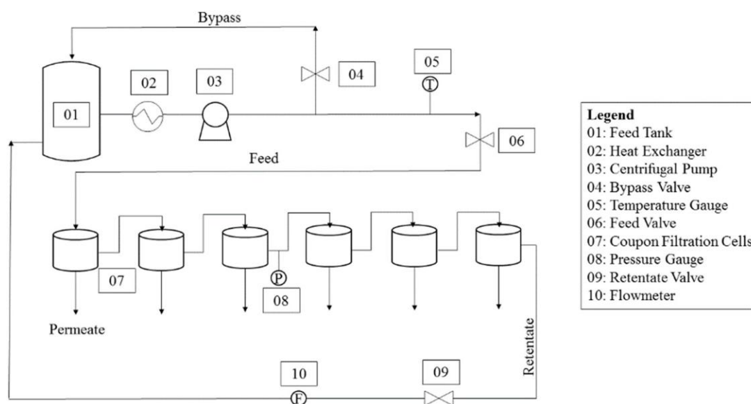
Figure 1. Cross flow nanofiltration setup.
