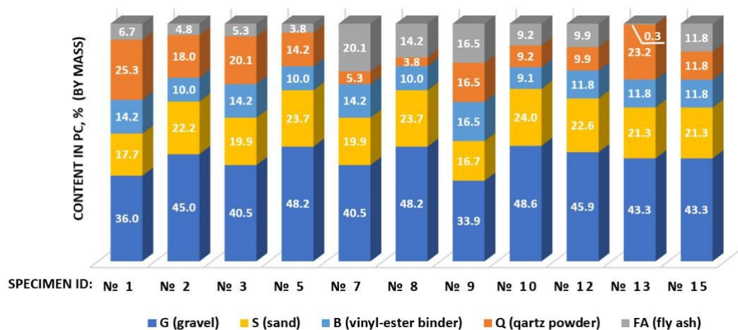
Figure 5. Vinyl-ester-concrete compositions (% by mass) based on the statistical Box design (experimental CCD design of three factors expressed as the mass ratios of components: B/(G+S) in the range of 0.0–1.0, B/(FA+Q) in the range of 0.0–1.0, and FA/(FA+Q) in the range of 0.0–1.0). Specimens tested in the presented research were the halves of prisms with dimensions of 40 \times 40 \times 160 mm 3 in were the halves of prisms with of 40 40 160 mm 3 after the flexural test (three-point bending test). The presented compressive 160 mm remaining after the flexural test (three-point bending test). The presented compressive
