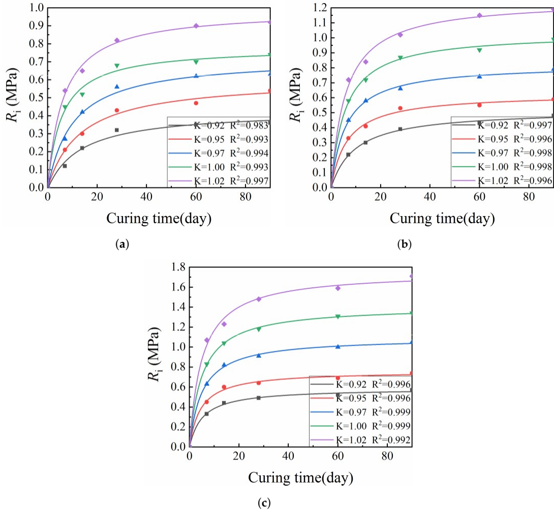
Figure 5. Relationship between curing time and splitting strength for cement-improved loess: (a) cement dosage 3%; (b) cement dosage 4%; (c) cement dosage 6%. The compaction coefficient K is the specimen of the specimen.
