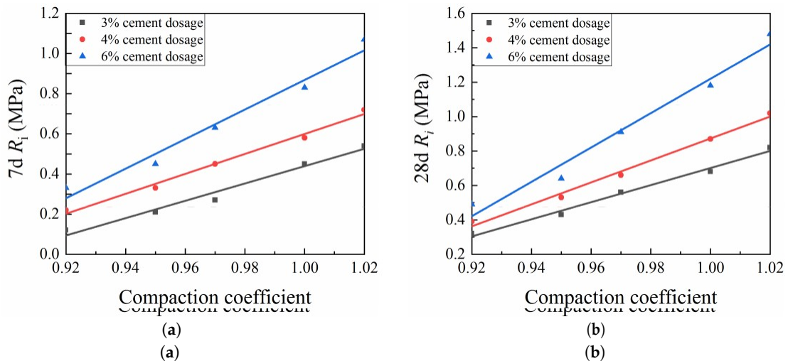
Figure 9. Relationship between compaction coefficient and splitting strength (SS) of cement-modified loess (CML): (a) seven-day (7d) SS; and (b) twenty-eight-day (28d) SS.
