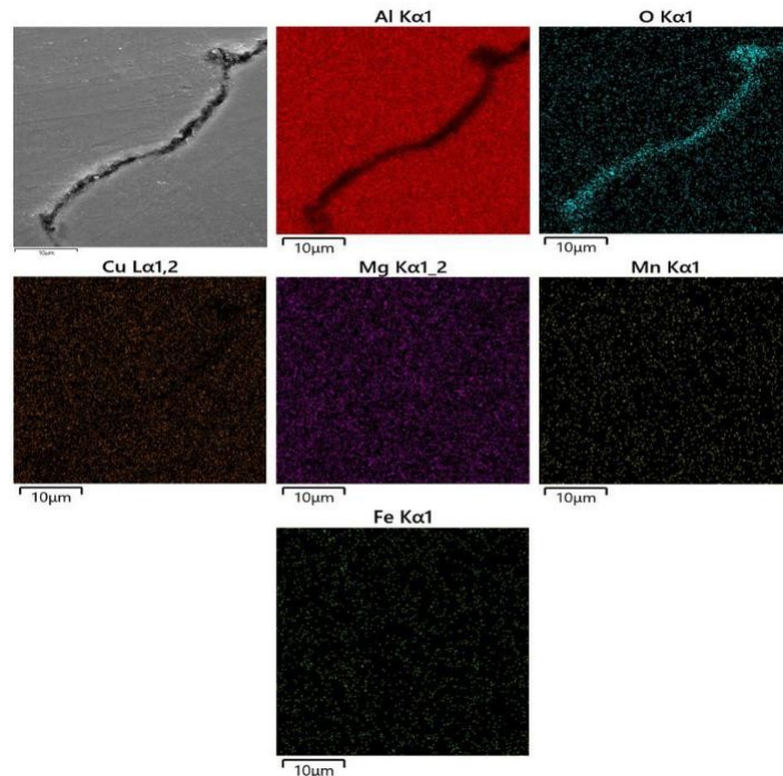
Figure 11. Energy Dispersive Spectroscopy (EDS) mapping analysis results for a crack of Al-rich oxide clusters
