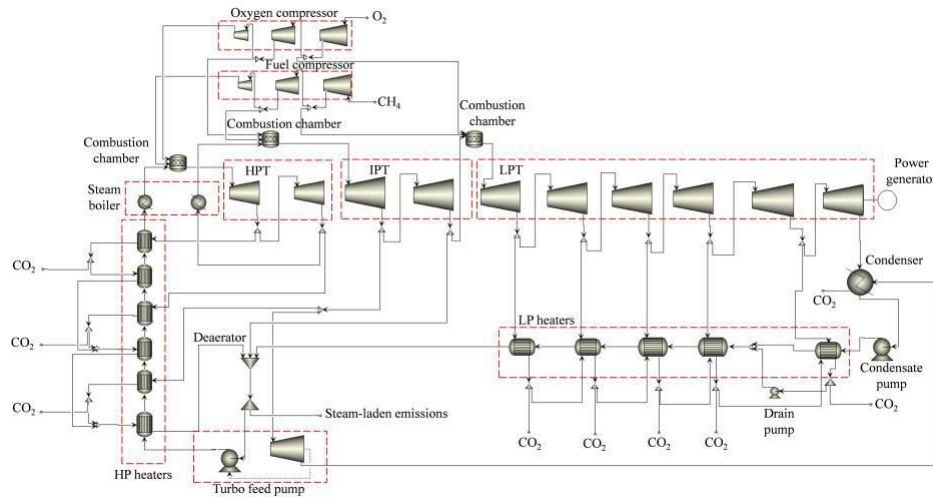
(b) double reheat
