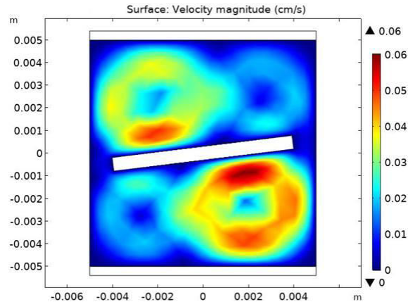
Figure 10: Velocity profile cooling: COMSOL, CO 2 inside skylight.
