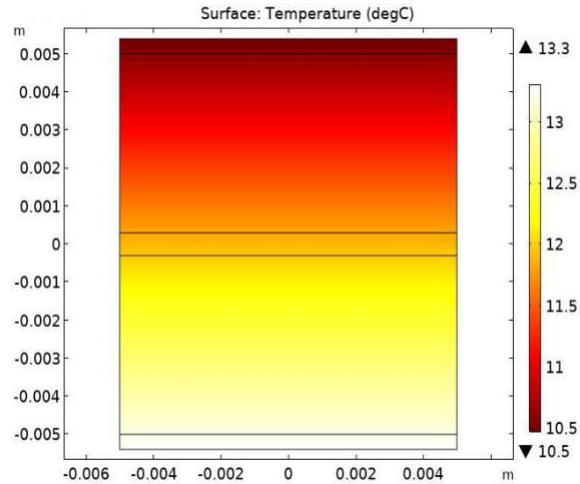
Figure 9: Temperature profile insulating: COMSOL, CO 2 inside skylight.
