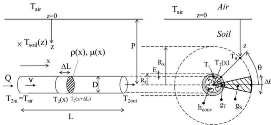
Figure 2: Description of the studied buried pipe used in the HeatGround software.
