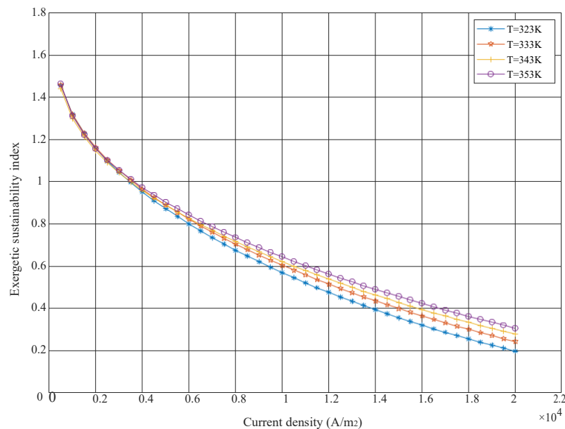
Figure 10: Variation of ESI as a function of current density, under varying operating temperatures when the operating pressure is fixed to 3.039 \times 10^5 Pa.
