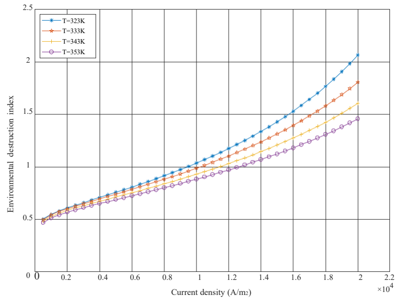
Figure 8: Variation of EDI as a function of current density, under varying operating temperatures when the operating pressure is fixed to 3.039 \times 10^5 Pa.
