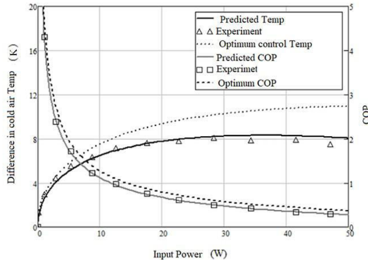
Figure 4: Variation of experiment and predicted coefficient of performance (COP) and cold air temperature difference against input power.
