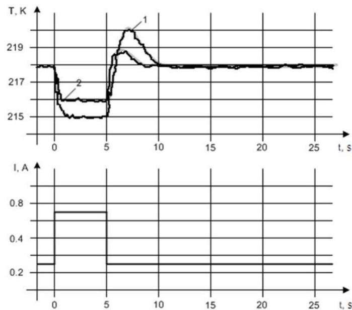
Figure 3: The results of a study of transients on a thermoelectric module 1MC06-030-05.
