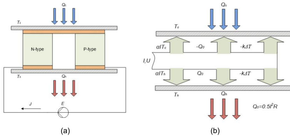
Figure 1: Model of an element of a thermoelectric battery based on the Peltier effect.
