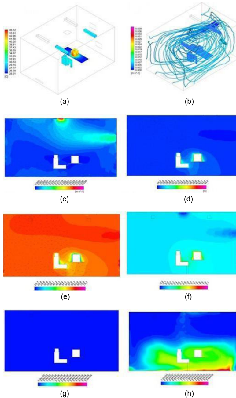
Figure 10: Effect of natural ventilation from the airflow window in the office for case NM4:
