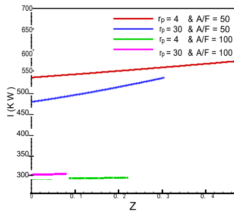
Figure 4: Variation of total exergy destruction with respect to partial amount ( z ) of the combustible gases for different pressure ratio ( r_p ) and air-fuel ratio ( A/F ).
