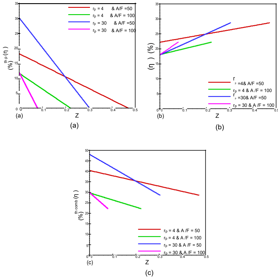
Figure 3: Variation of thermal efficiency of primary cycle (a), secondary cycle (b), and combined cycle (c) with respect to partial amount (z) of the combustible gases for different pressure ratio ( r_p ) and air-fuel ratio ( A/F ).
