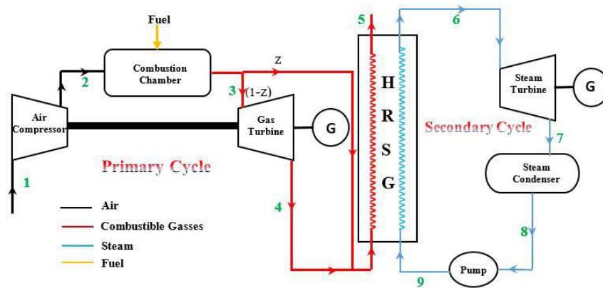
Figure 1: Schematic diagram of proposed cycle under study: G – electric generator, HRSG – heat recovery steam generator, Z – partial amount of the combustibles gases.
