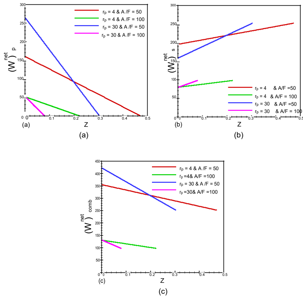
Figure 2: Variation of network output of primary cycle (a), secondary cycle (b), and combined cycle (c) with respect to partial amount ( z ) of the combustible gases for different pressure ratio ( r_p ) and air-fuel ratio ( A/F ).
